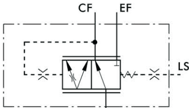
Static signal PRT.../40,80...; PRTA.../40,80...
